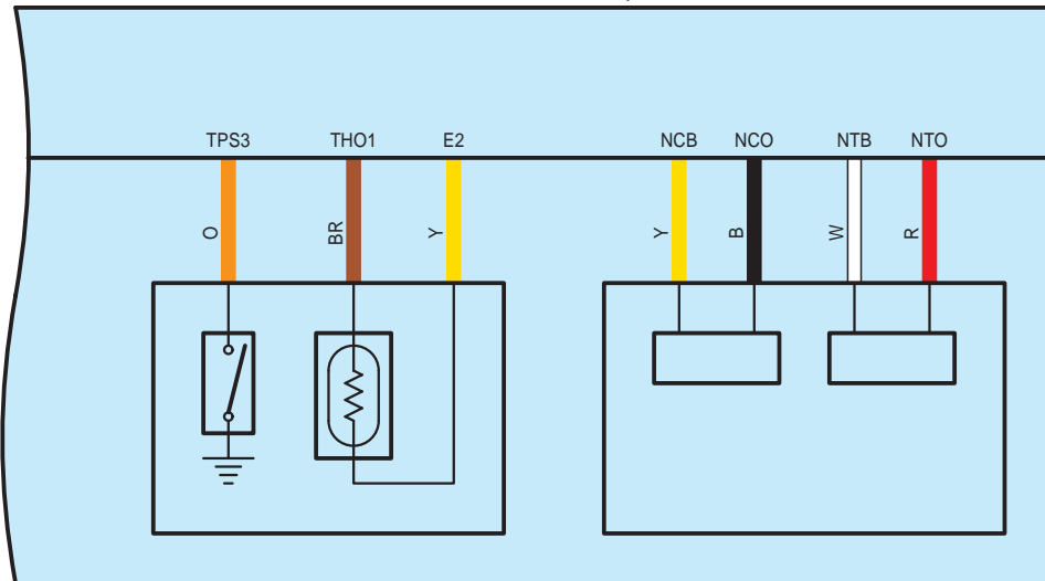
B2 Transmission Control ECU Assembly
