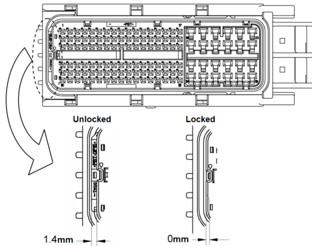
Connector Locking detail
